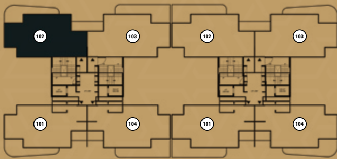
KEY PLAN - TOWER C1/C2 TYPICAL FLOOR
